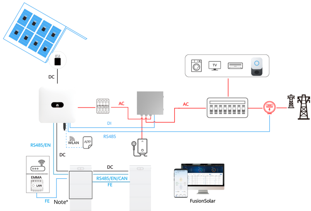
Figure 2-8 On/Off-grid scenario
