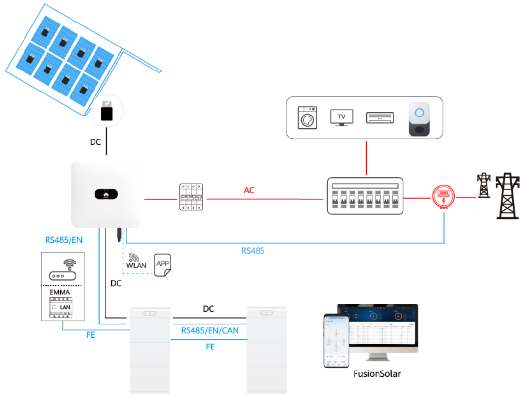
Figure 2-7 On-grid scenario
